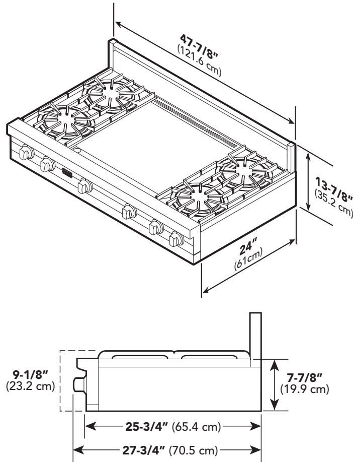
VGRT482-4G 48"W. Four-Burner/ Double Griddle Rangetop
