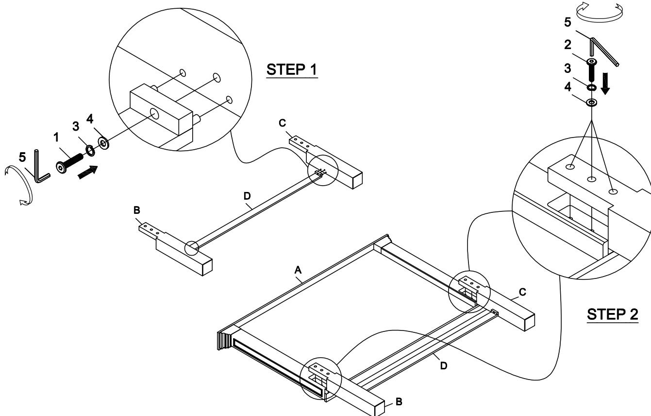
Complete Assembly
