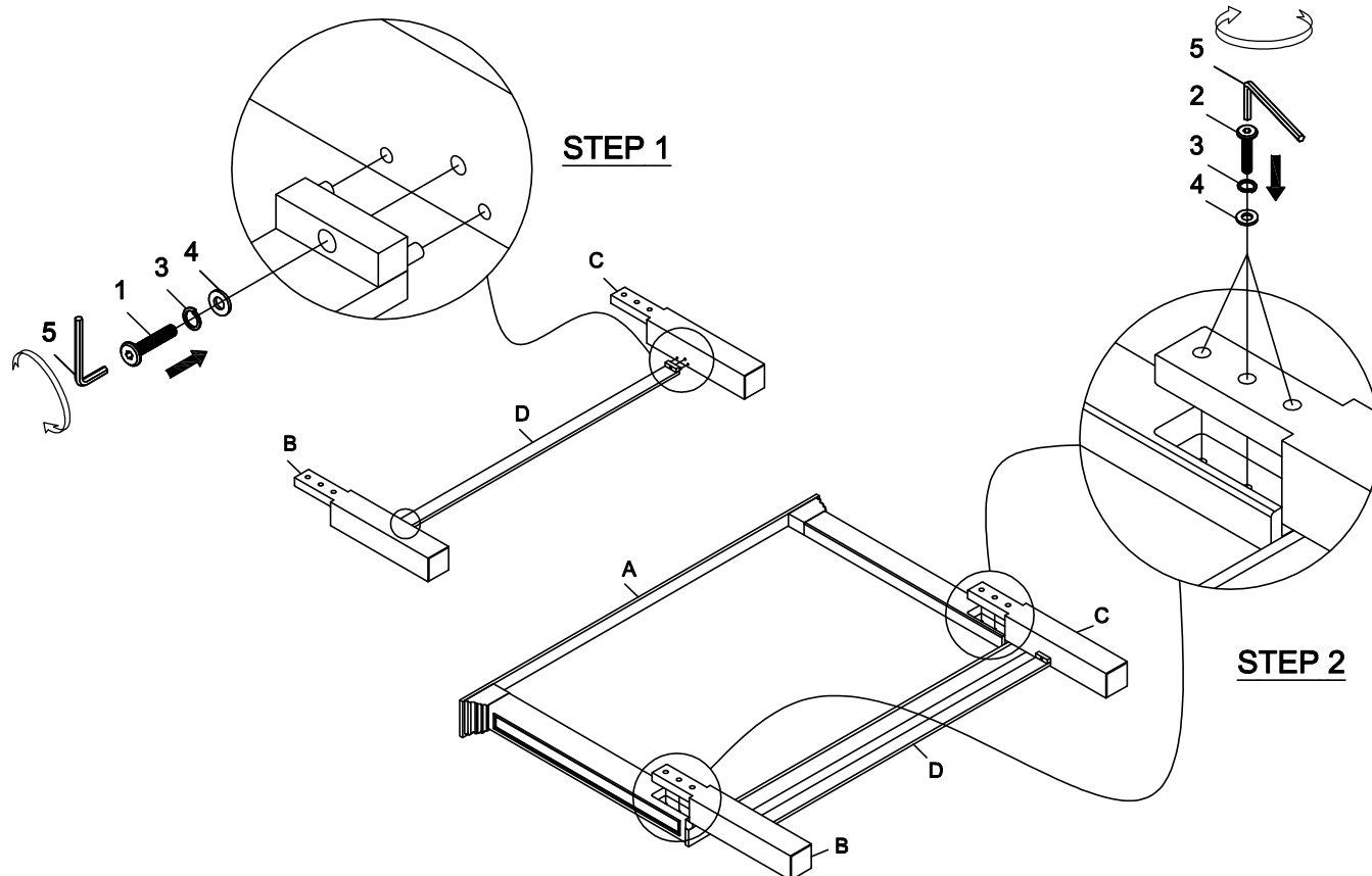
Complete Assembly
