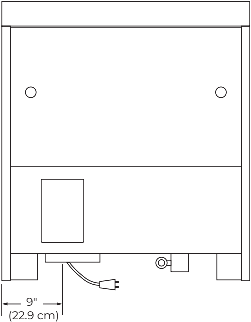
BACK VIEW
