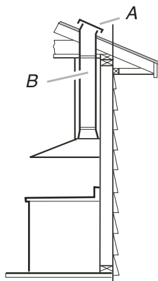
A. Roof cap B. 10" (25.4 cm) round vent
