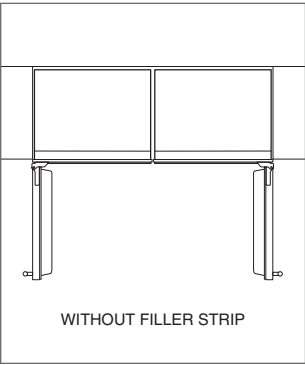
Opposite hinges
