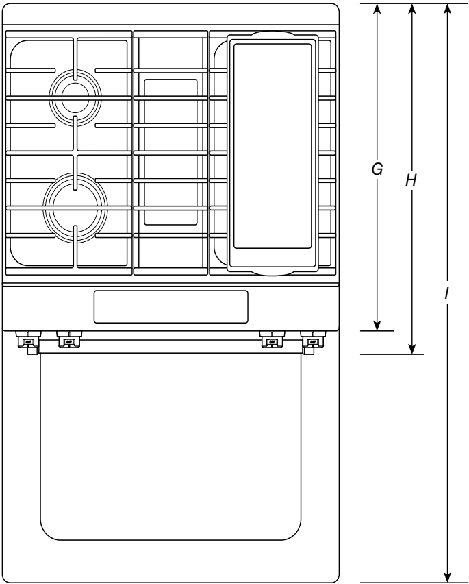
TOP VIEW
