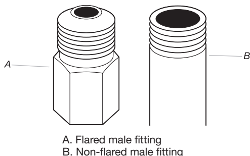
B. Non-flared male fitting
