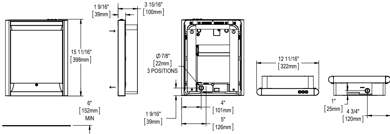
DEVANT | FRONT
