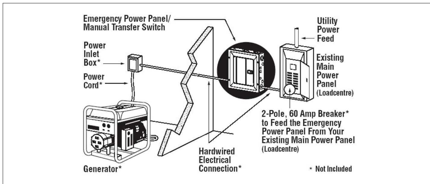
Figure 20. Typical installation diagram
