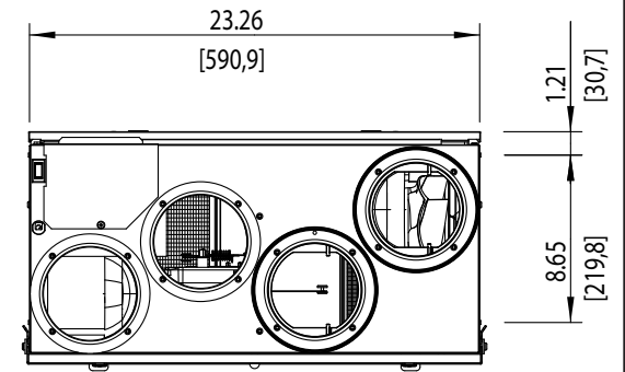
(Ceiling Chain) Hanging Hole Pattern Top View
