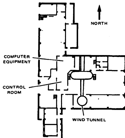
3.5-ft WIND TUNNEL FLOOR PLAN
