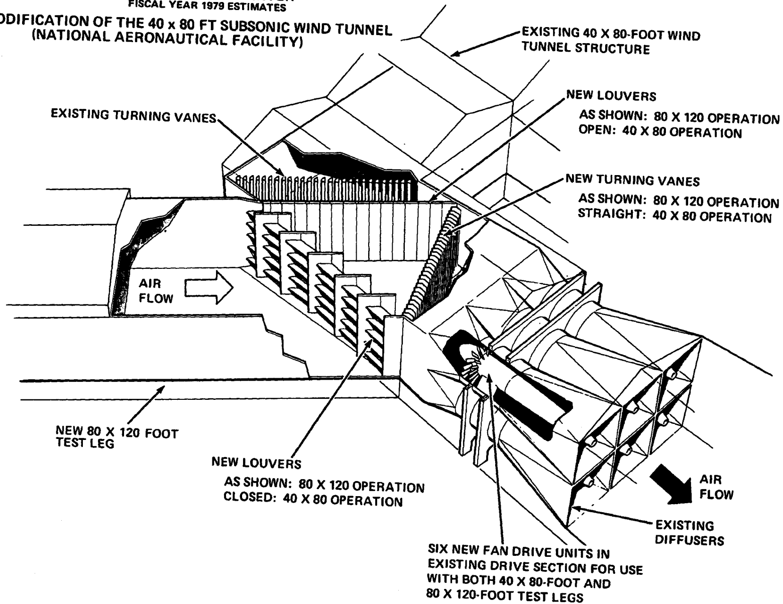
PERSPECTIVE VIEW OF VANES, LOUVERS, AND FAN DRIVE SYSTEM
