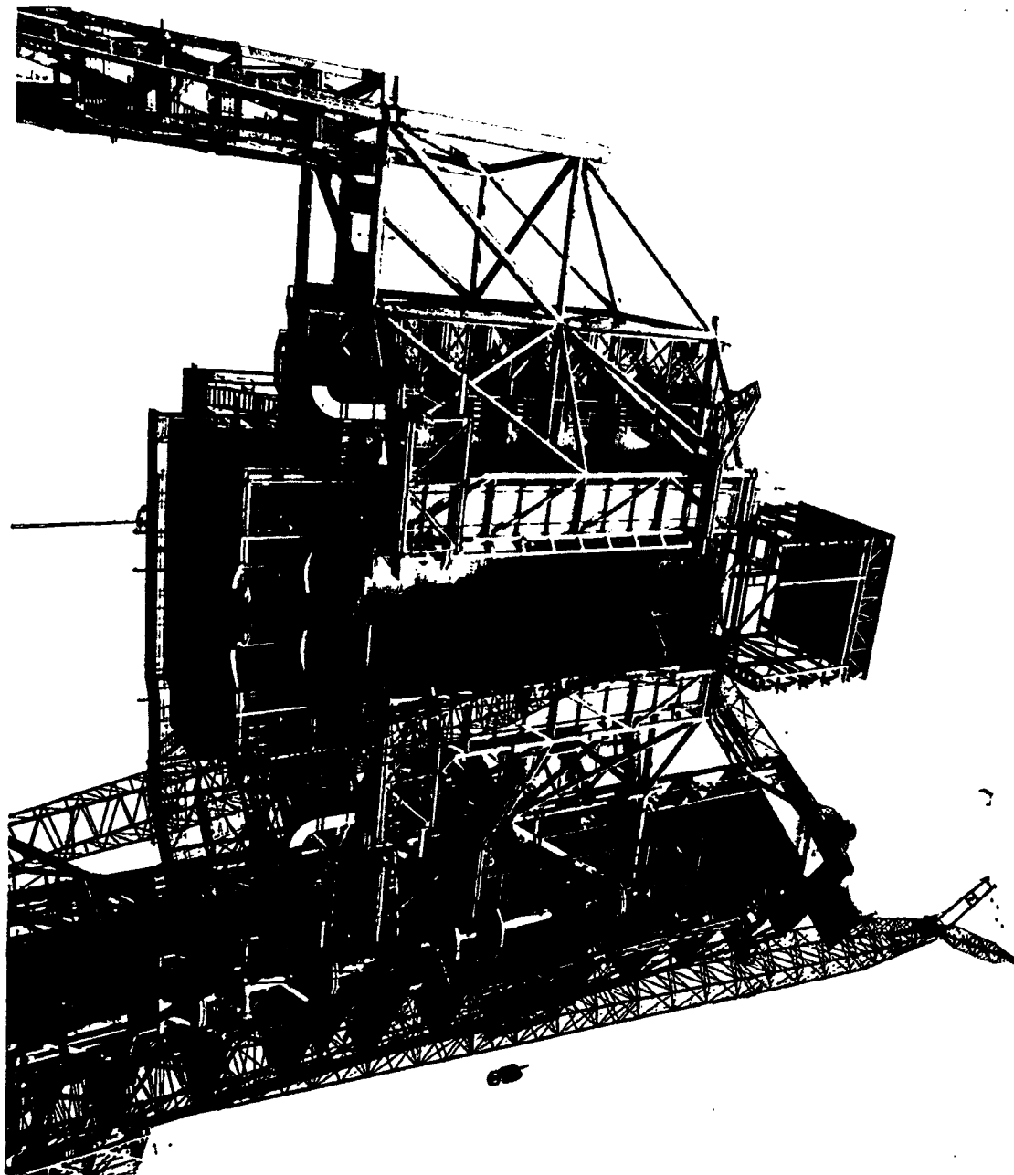
PAYLOAD CHANGEOUT ROOM (SHOWN IN RETRACTED POSITION AT PAD "A")
