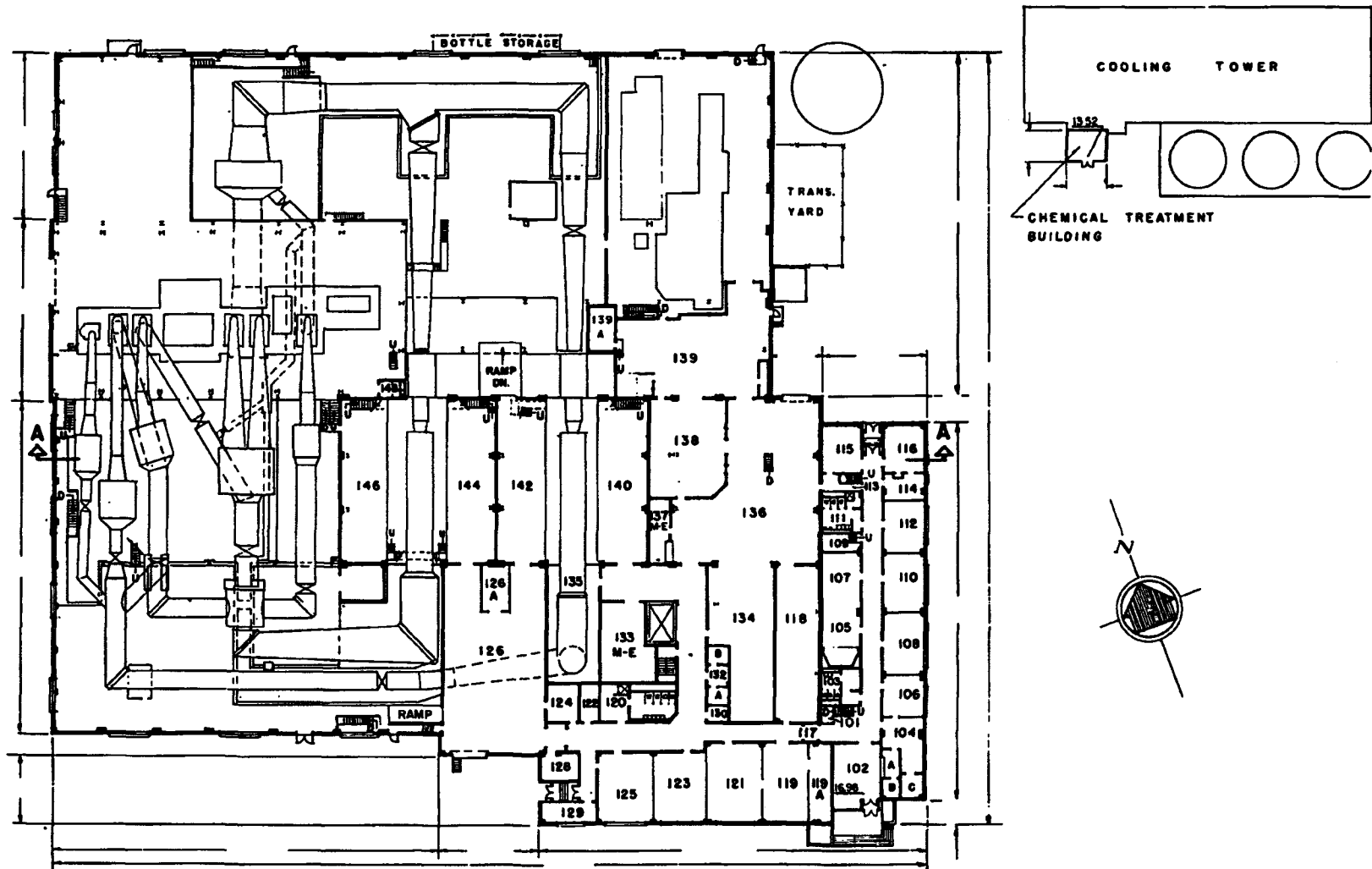
FIRST FLOOR PLAN FIGURE 3
