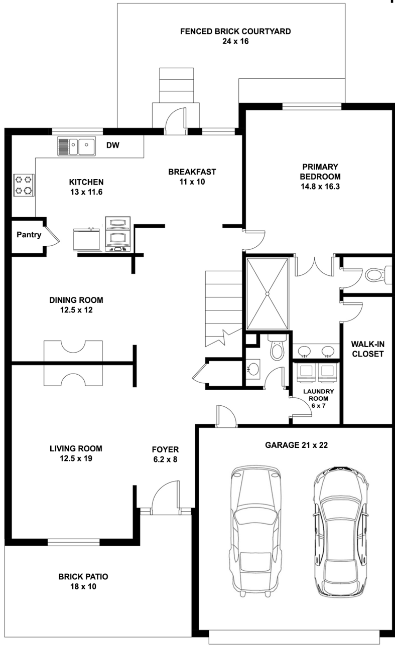
FIRST FLOOR
