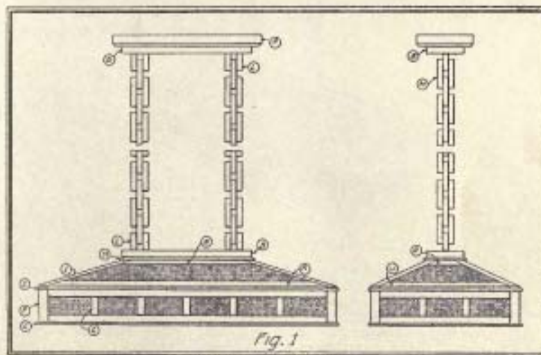
Side and End Views of Dome.
