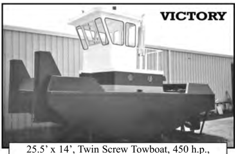
25.5' x 14', Twin Screw Towboat, 450 h.p., 3.5' Draft.
