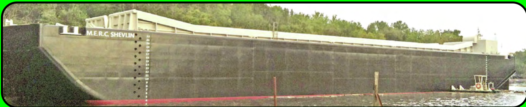
5,000 ABS All Oceans Cubic Yard Split Hull Dump Scow - Located in FL
