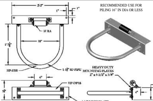
HP-H18 18" Hoop 14# $56.26 H-RA Roller Assembly 5# $25.67 HP-DP18 Deck Plate 18# $43.94 HP-H18R Assembly Complete 37# $125.87
