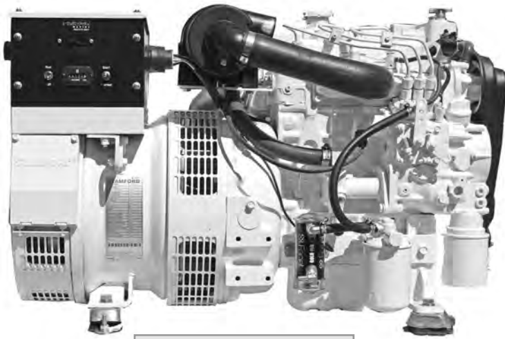
K3 - 9.5 KW
