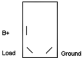
RS1071 Rocker Switch
