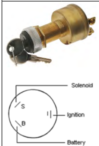
SW63 Ignition Switch with Lock Cylinder
