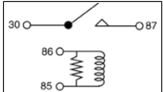
AR620 ABS Relay 4740114; 4707072; 4687143
