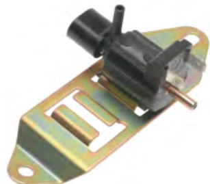
2-282616 Canister Purge Solenoid G622-18-740
