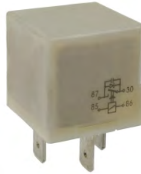
AR7213 A/C Auto Temp Control Relay 443 919 578C
