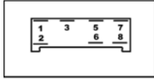
AR727 Computer Control Relay RZ-0088; 39400-SM4-003; 39400-SL5-A01; 39400-SV4-003
