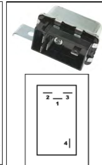
AR704 A/C Compressor Clutch Cut-Off Relay 4419200 Chrysler..... 1991 - 1988 Dodge..... 1990 - 1988 Plymouth..... 1991 - 1987
