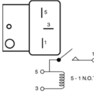
HR126 Horn Relay
