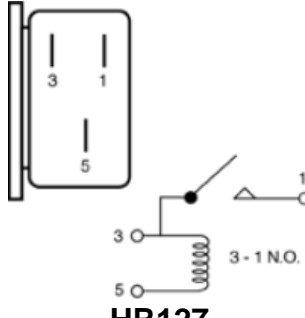
HR127 Horn Relay
