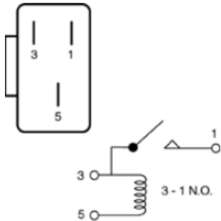
HR123 Cruise Control Relay
