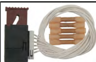
EC516 Accelerator Pedal Sensor Connector 89046653
