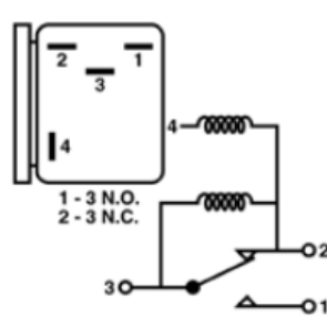
HR131 Engine Temperature Warning Buzzer Relay 1115867
