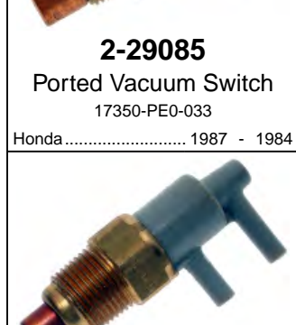
2-29085 Ported Vacuum Switch 17350-PE0-033 Honda ..... 1987 - 1984
