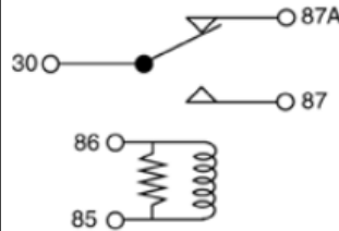
AR617 Multi-Function Relay 56007203; 4687147
