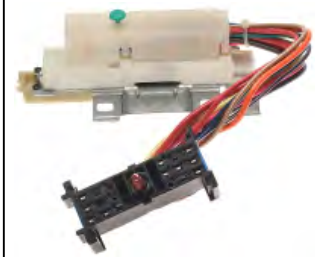
KS6192 Ignition Starter Switch 26009611 Buick ..... 1989 Cadillac ..... 1993 - 1989
