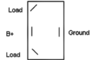
RS1073 Rocker Switch
