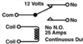
AR211 A/C and Heater Delay Relay
