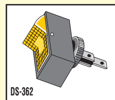
Rocker Switch Universal, heavy duty, illuminated rocker switch. Mounting 1/2" round hole, illuminated in "ON" position. Rating: 20 Amp. 12 Volt. DS-362 - Amber Illuminated DS-364 - Red Illuminated DS-365 - Non-Illuminated DS-1821 - Green Illuminated
