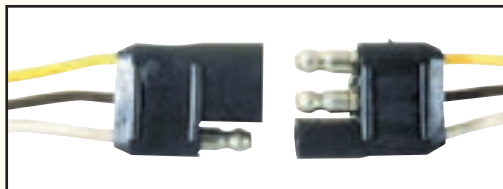
TC30 3-Pole Molded Trailer Connector • 18 gauge pigtails for boats, trailers, etc. • Plug and receptacle are not sold separately
