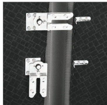
Included quick connect/disconnect hardware swivels out of sight when not in use
