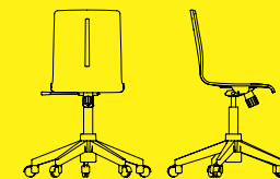
PL40/41/42 BW 15.5" SW 16.25" BH 16.5" SH 17-20.5" SD 15"
