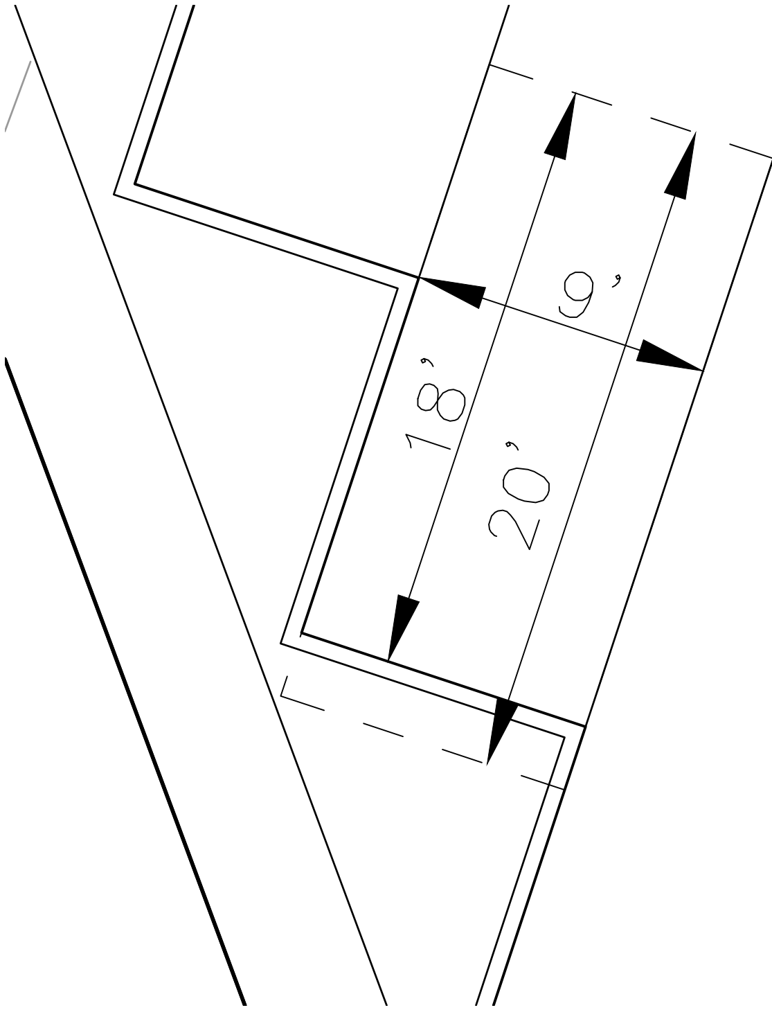
TYPICAL PARKING SPACE DETAIL NOT TO SCALE
