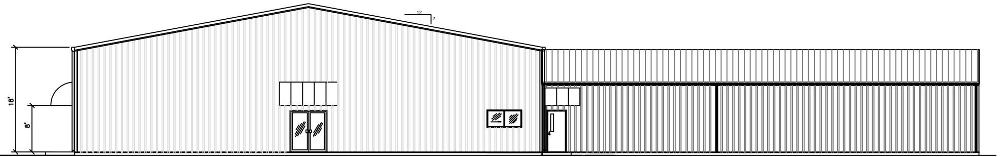
WEST ELEVATION
