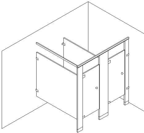
academy FLOOR MOUNTED OVERHEAD BRACED
