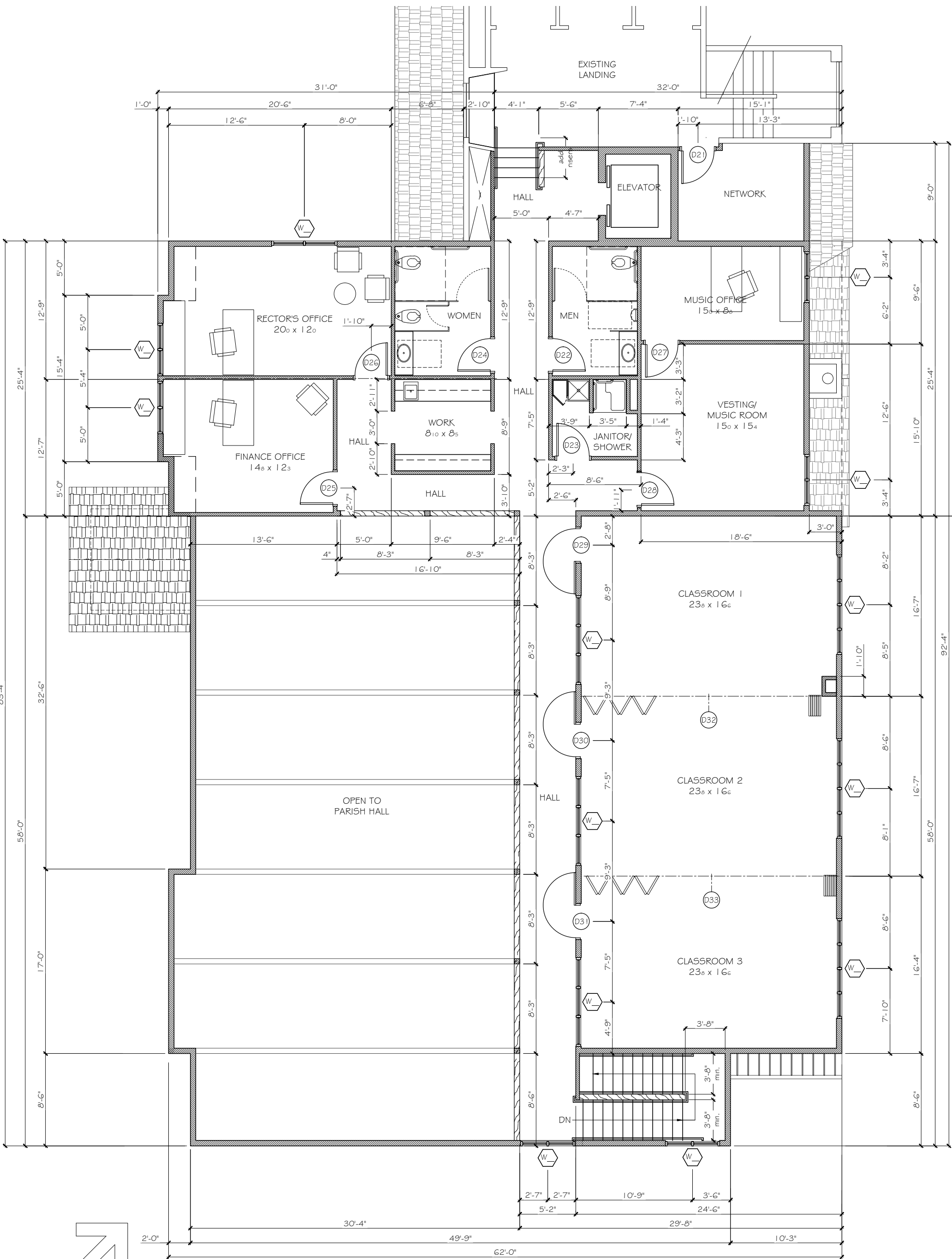
2 PROPOSED SECOND FLOOR PLAN SCALE: 3/16"=1'-0"
