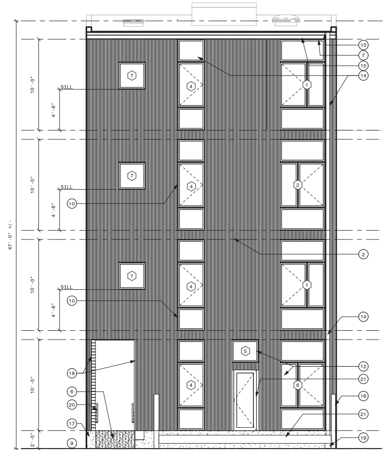
REAR ELEVATION
