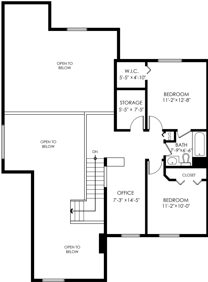
Upper Floor Plan Floor Area: 734 sq.ft. Ceiling Height: 8'
