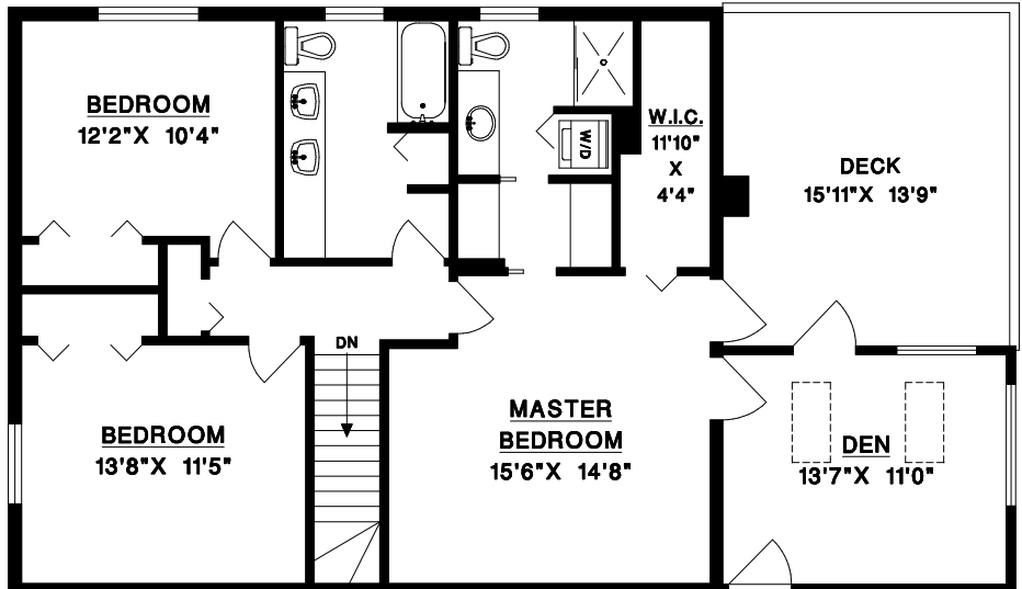
UPPER LEVEL
