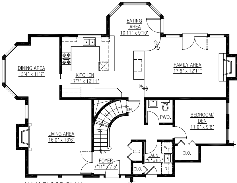
MAIN FLOOR PLAN FLOOR AREA: 1,383 sq.ft.
