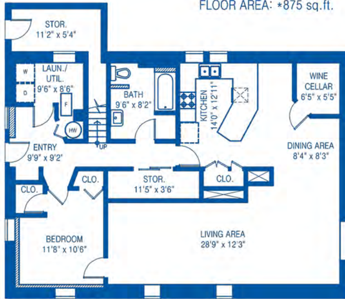
BASEMENT FLOOR PLAN FLOOR AREA: 1,276 sq.ft.
