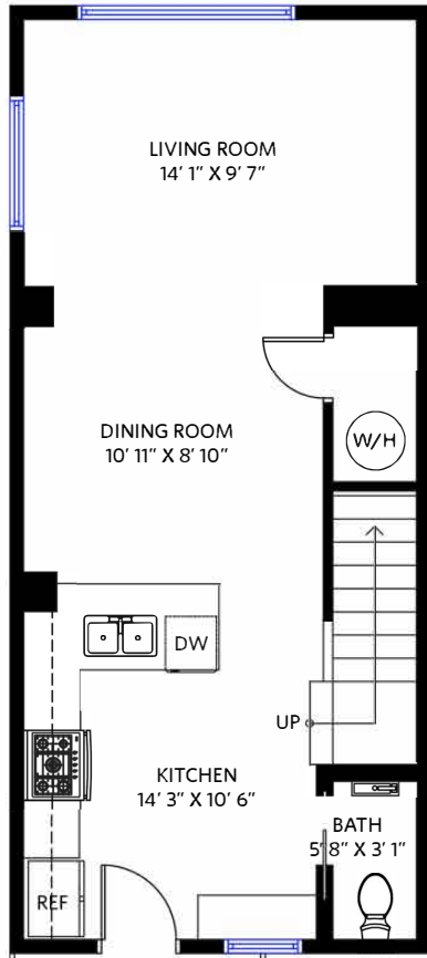
Main Floor: 513 Sq.Ft. Ceiling Height: 9'2"
