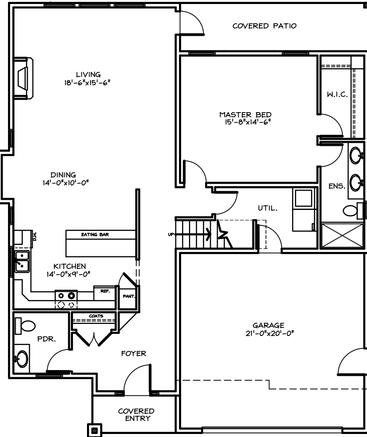
MAIN FLOOR PLAN 1356 SQ. FT. 2159 SQ. FT. TOTAL
