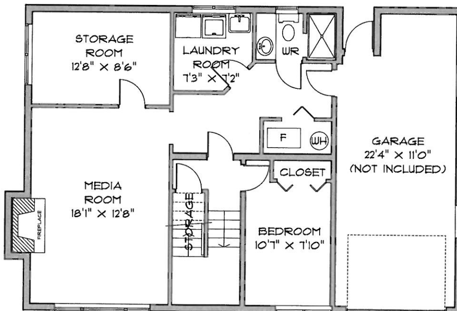
LOWER LEVEL 817 SQ. FT.
