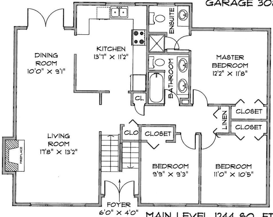
MAIN LEVEL 1244 SQ. FT.
