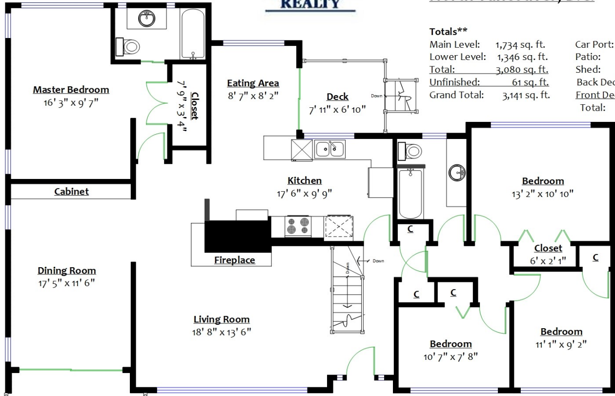
MAIN LEVEL Floor Area: 1,734 Sq. Ft.
