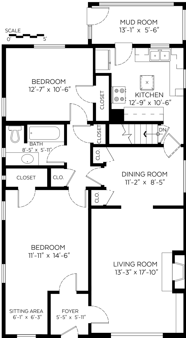
Main Floor Plan Floor Area: 1,122 sq.ft.
