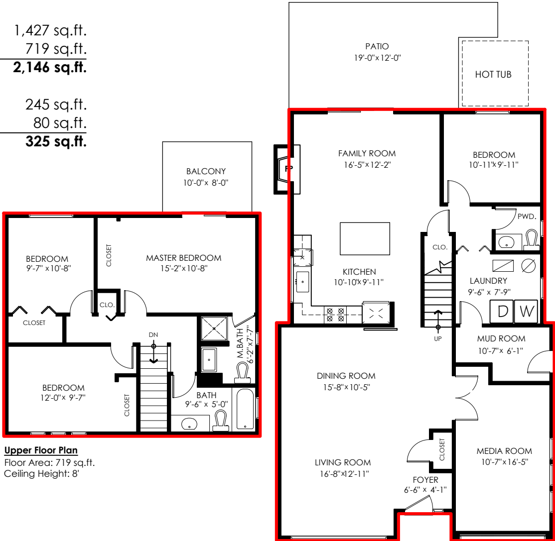
Main Floor Plan Floor Area: 1427 sq.ft. Ceiling Height: 8'
