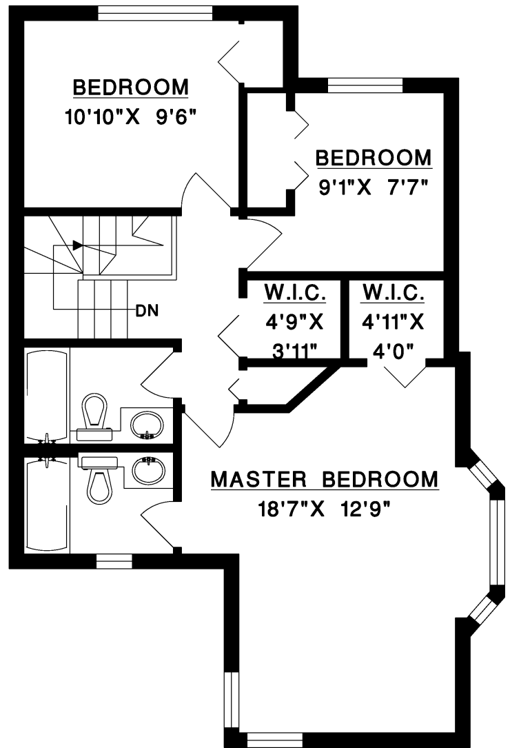
UPPER FLOOR
