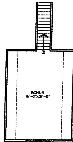
BONUS PLAN 368 SQ. FT.
