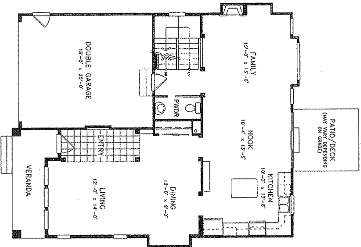
MAIN FLOOR PLAN 1080 SQ.FT. GARAGE: 378 SQ.FT.
