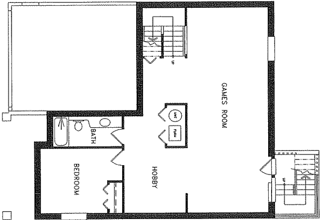
BASEMENT FLOOR PLAN 1067 SQ. FT. (SHOWING OPTIONAL FINISHED BASEMENT. PATIO, WINDOWS AND DOORS MAY VARY.)
