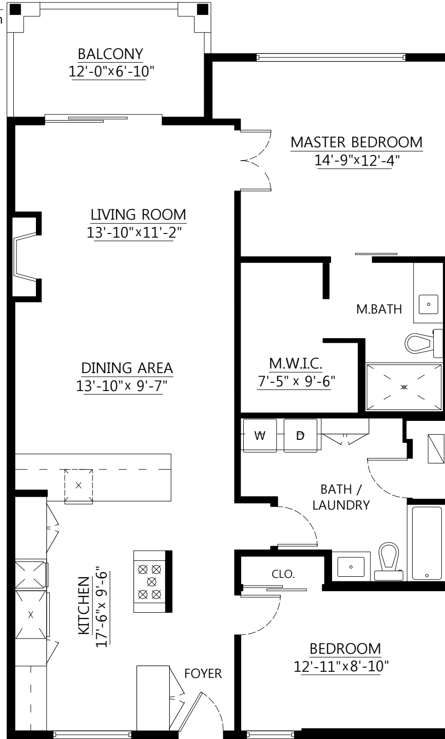
Main Floor Plan Floor Area: 1,168 sq.ft.
