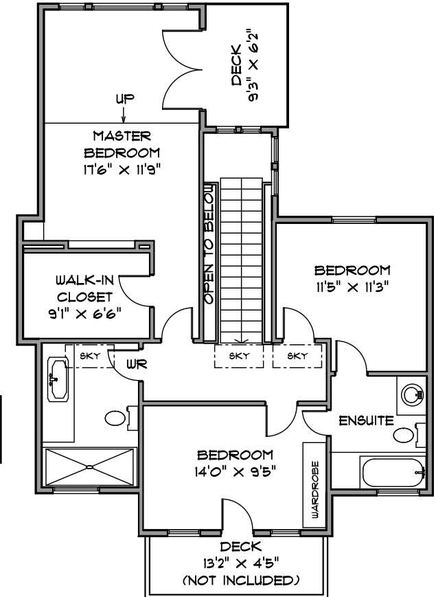
UPPER LEVEL 940 SQ. FT.
