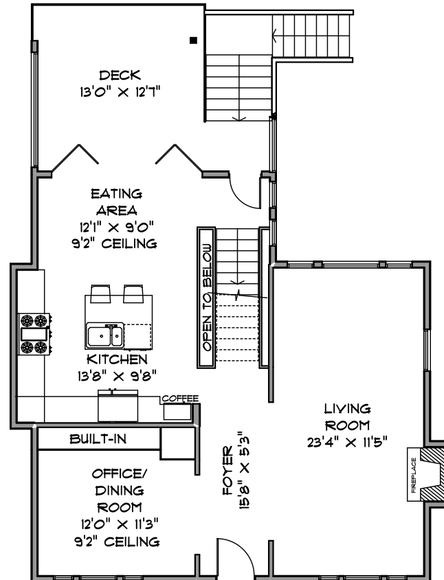
MAIN LEVEL 892 SQ. FT.
