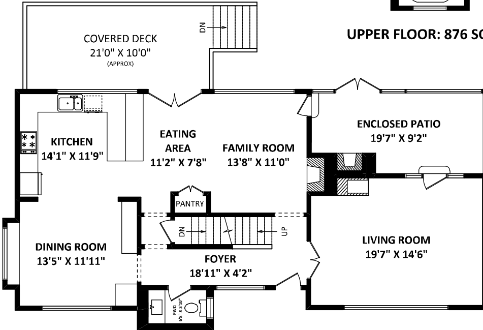
MAIN FLOOR: 1346 SQ.FT.
