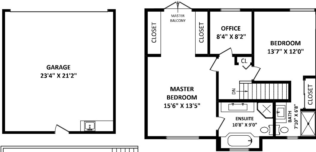
UPPER FLOOR: 876 SQ.FT.
