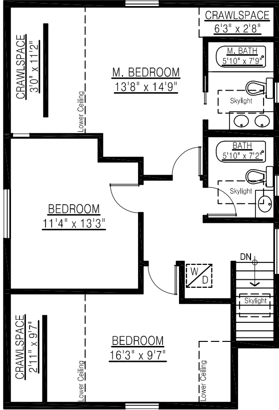
UPPER FLOOR PLAN FLOOR AREA: 750 sq.ft.
