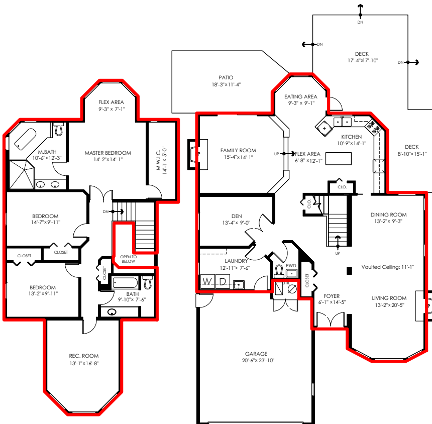
Upper Floor Plan Floor Area: 1322 sq.ft. Ceiling Height: 8'
