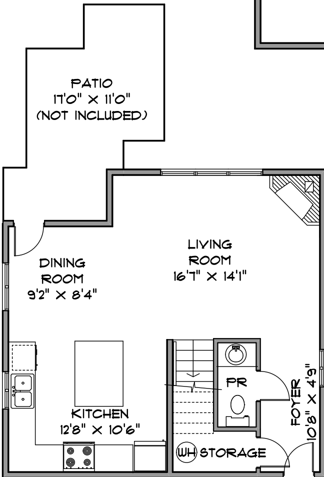
MAIN LEVEL 607 SQ. FT.
