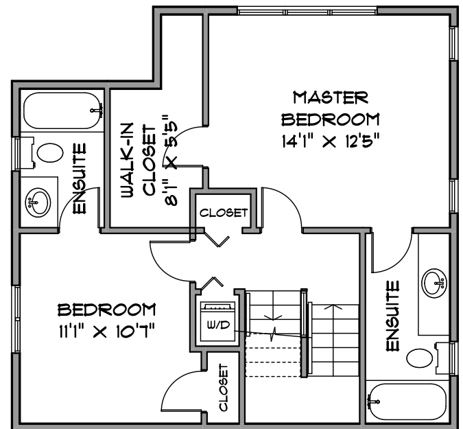
UPPER LEVEL 612 SQ. FT.
