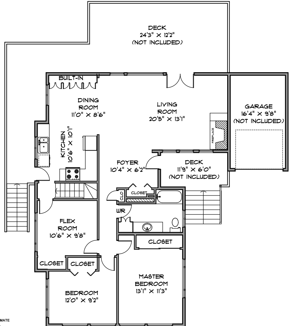
MAIN LEVEL 1233 SQ. FT.
