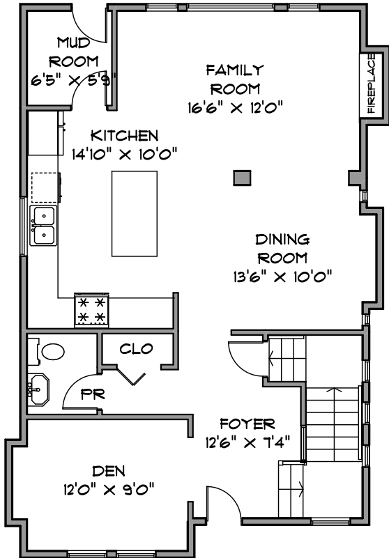
MAIN LEVEL 887 SQ. FT.
