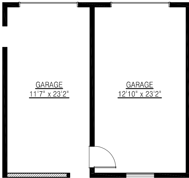
GARAGE PLAN FLOOR AREA: 637 sq.ft.
