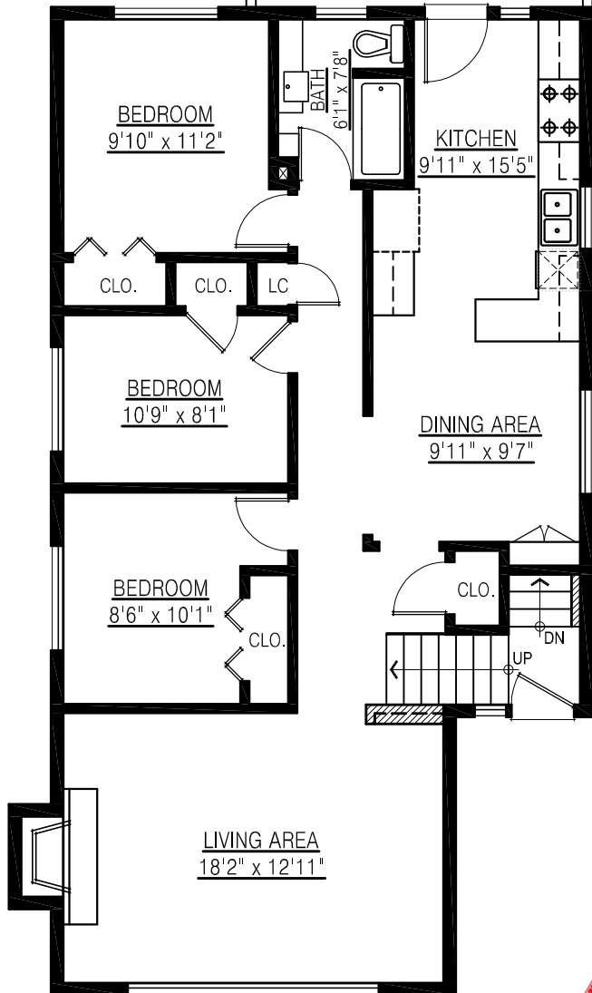
MAIN FLOOR PLAN FLOOR AREA: 1,134 sq.ft.
