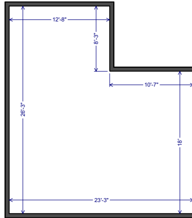
MAIN LEVEL
