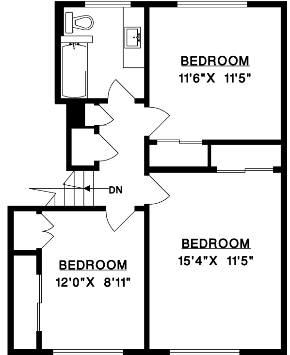
UPPER FLOOR
