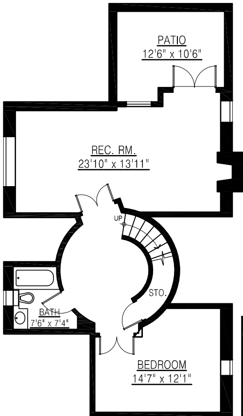
LOWER FLOOR PLAN FLOOR AREA: 928 sq. ft.
