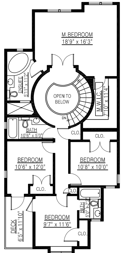
UPPER FLOOR PLAN FLOOR AREA: 1,229 sq. ft.
